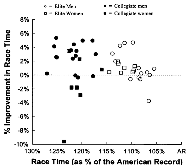
Fig. 4. Comparison of athletes of various performance levels and the change in performance from a 4-wk living high-training low altitude sojourn. Race time represents the initial time trial presented as a percent of the American record (AR) in the event at the time. The change in performance is the percent change from the precamp time trial to the postcamp time trial.
